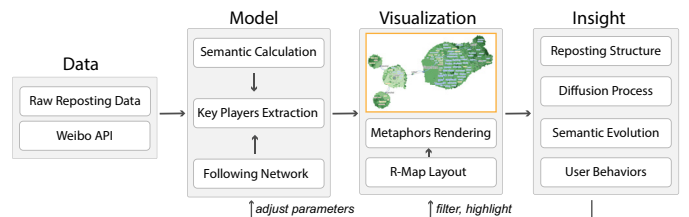
Fig. 7. Workflow of the R-Map visualization system.
